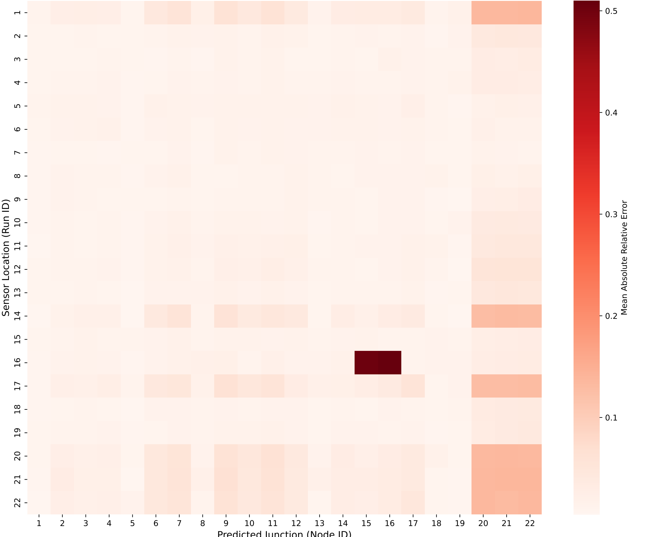
Anytown: Predictive Error by Single Sensor Placement
